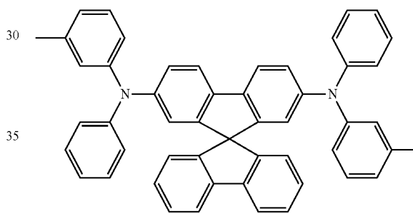
Spiro-TPD
