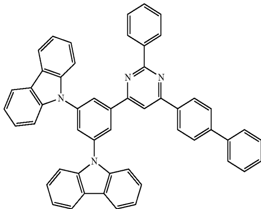
105 -continued
