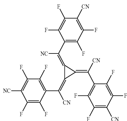
F4-TCNQ
