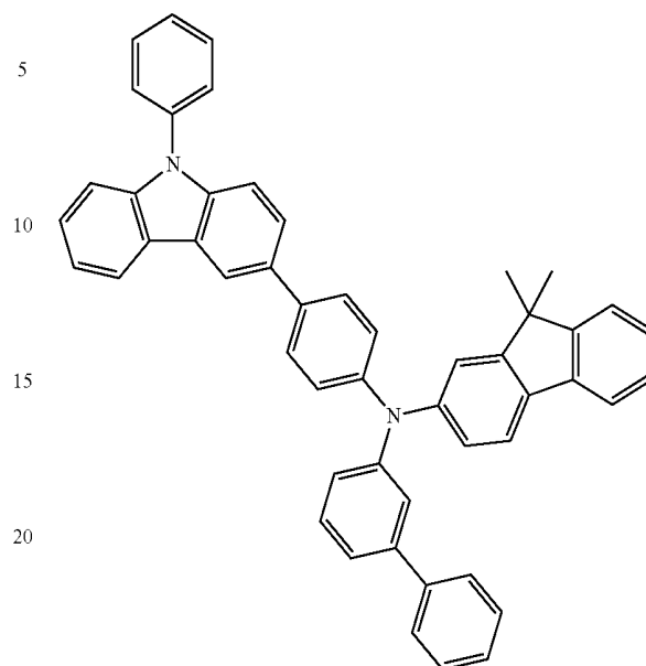
Formula 201A
