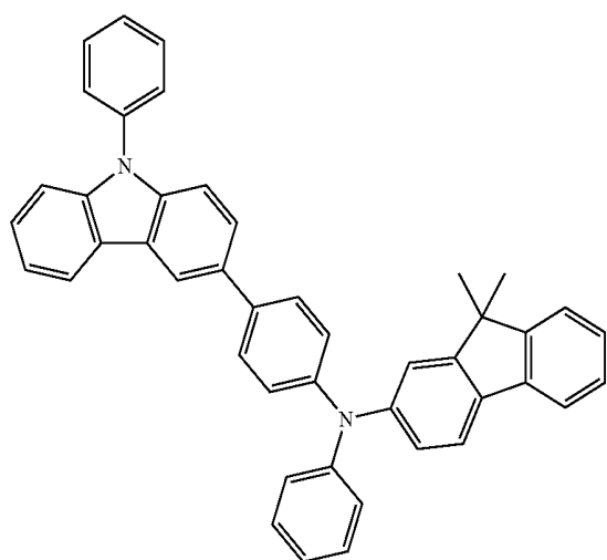
HT1
