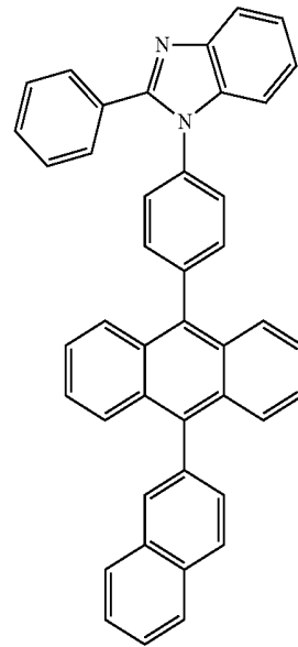
106 -continued
