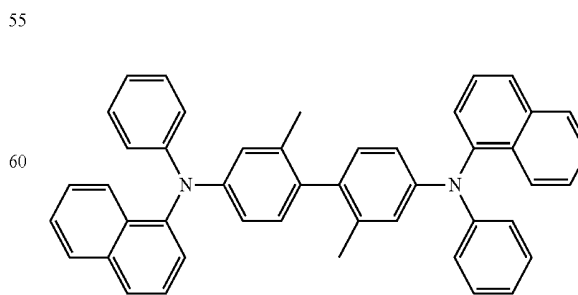
methylated NPB
