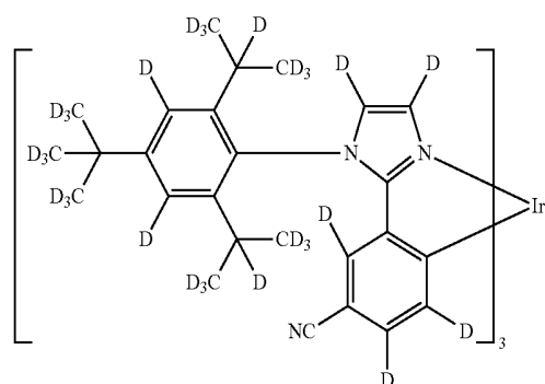
BD064
