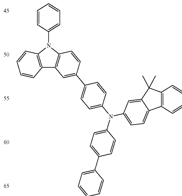
HT1
