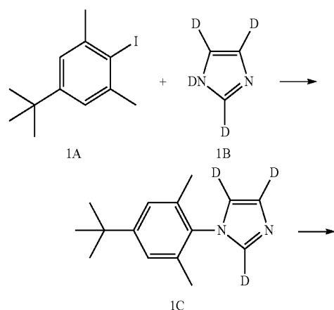
Reaction Scheme 1
