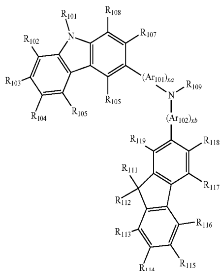
HMTDP
