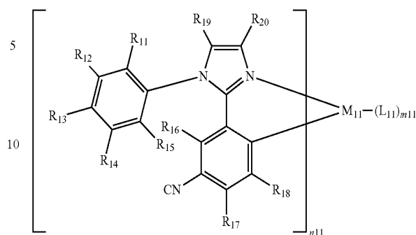
Formula 1
